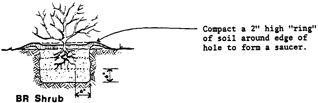
Figure 3-2. Planting methods.
